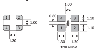
SOLDER PAD LAYOUT
